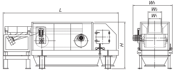
<Outline drawing of BMR-C casing included>
