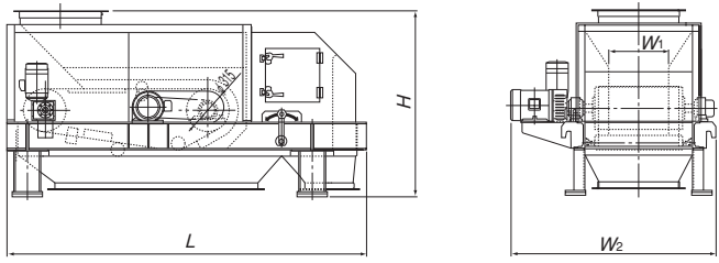
<Outline drawing of aluminum separator>
